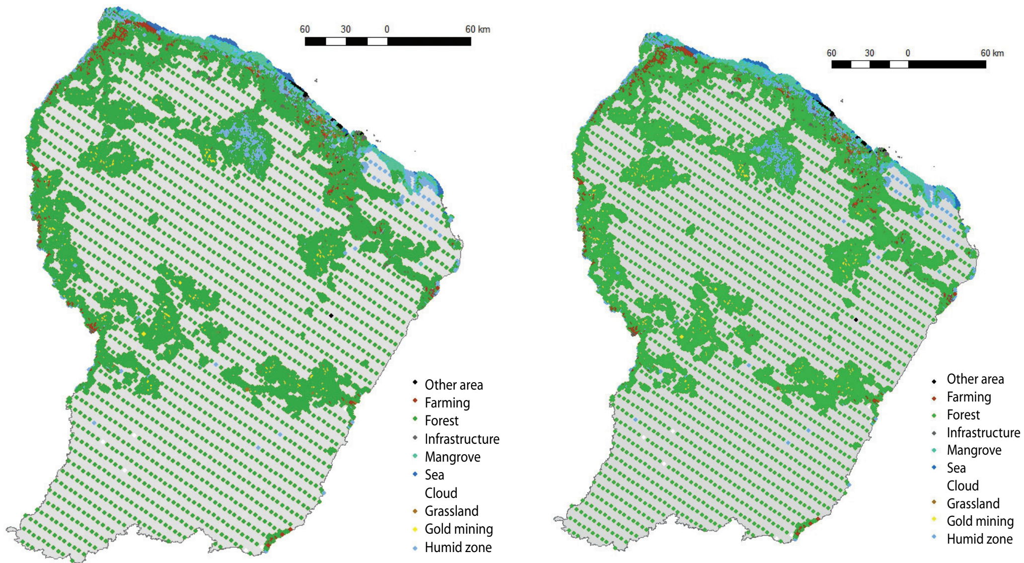
Fig 4. Comparison between 1990 (to the left) and 2012 (to the right) in terms of the spatial distribution of photo-interpreted plots
