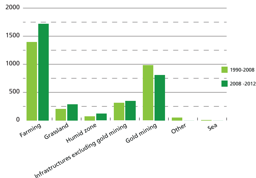
Fig 7. Annual flows from forest to other types of land cover between 1999 and 2008 and from 2008 to 2012
